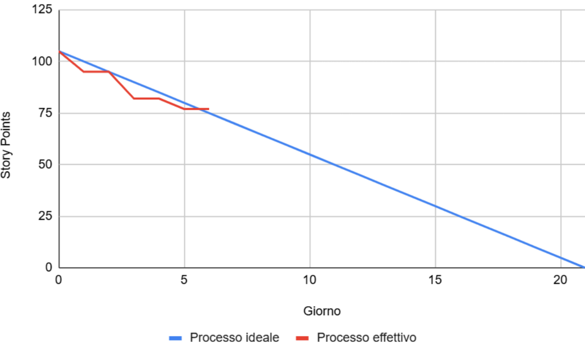
Burndown Chart
